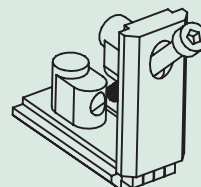
Escuadra hoja 7003 Ref. 2501502000
